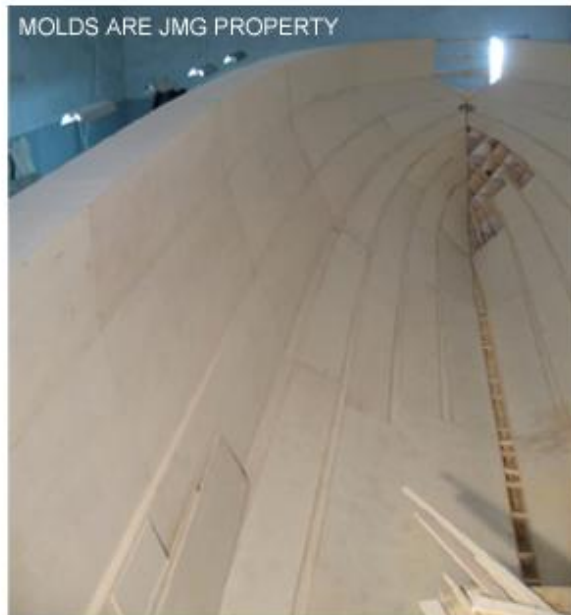
PILOT BOAT 12 MOLD CONSTRUCTION HULL
