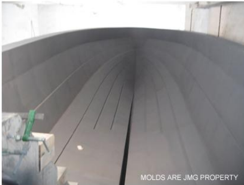
PILOT BOAT 12 MOLD CONSTRUCTION HULL
