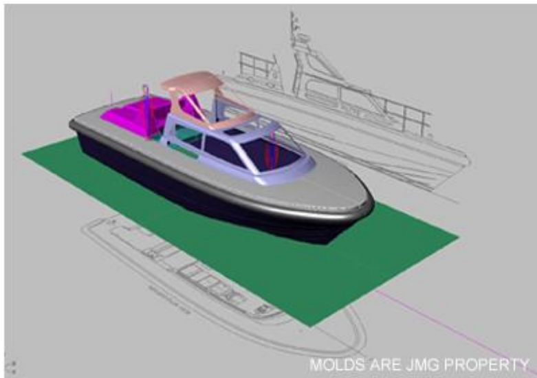
PILOT BOAT 12 DESIGN
